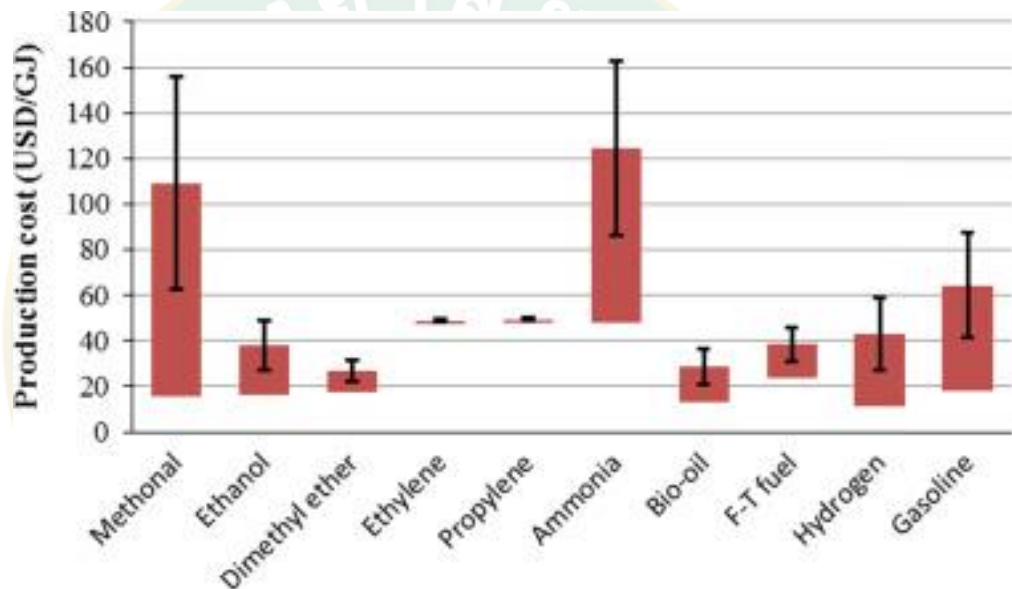
Figure 11 Comparison of chemical/fuels production cost
