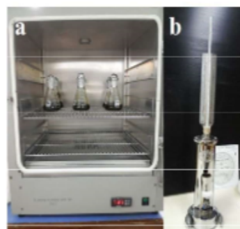
Fig. 3. Batch bioethanol experiment (a), Ebulliometer (b).
