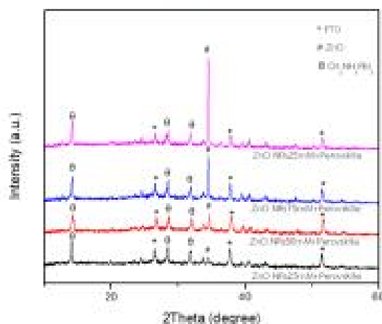
Fig. 5. XRD patterns of perovskite film fabricated on ZnO NRs growth from 4 different concentration.
