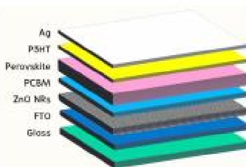
Fig. 1. Structure of perovskite solar cell that used in this work.
