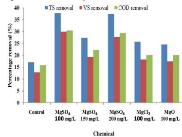
Figure 6. TS, VS and COD removal in anaerobic digestion for 15 days.
